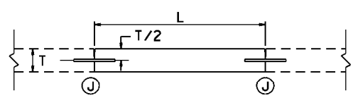
SECTION B MID-SLAB REPLACEMENT
