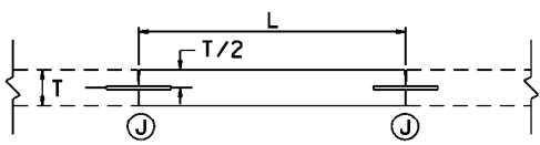
SECTION BB MID-SLAB REPLACEMENT
