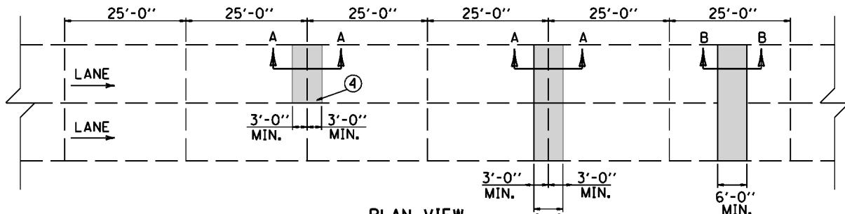
PLAN VIEW
