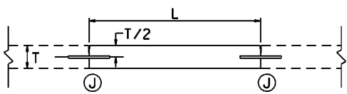
SECTION AA JOINT REPLACEMENT
