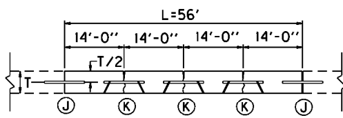
SECTION DD FULL WIDTH REPLACEMENT (INCLUDING JPC SHOULDERS)
